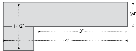
COLORADO STYLE (4" wide overall, 1-1/2" overhang)
