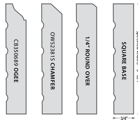
BASEBOARD (4' and longer, 3" to 7" specified widths, 3/4" thickness, side profiles shown)
