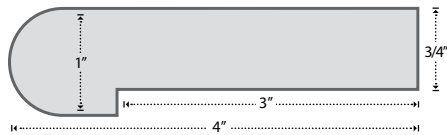
NOSING (4" wide overall, 1" overhang)
